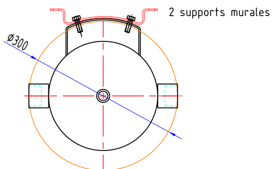
STA PUFFER 25 L mural 8 piquages
