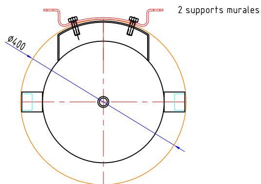
STA PUFFER 50 L mural 8 piquages
