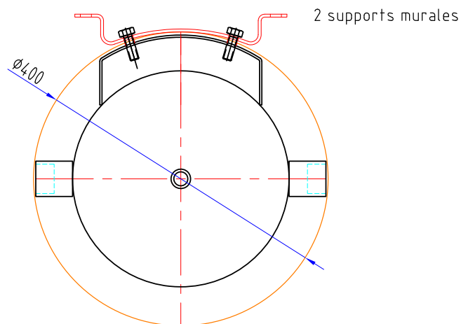
STA PUFFER 25 L mural 4 piquages
