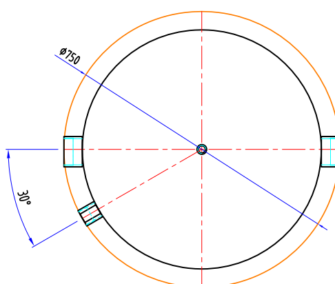
STA PUFFER 500 L sol/mural 8 piquages
