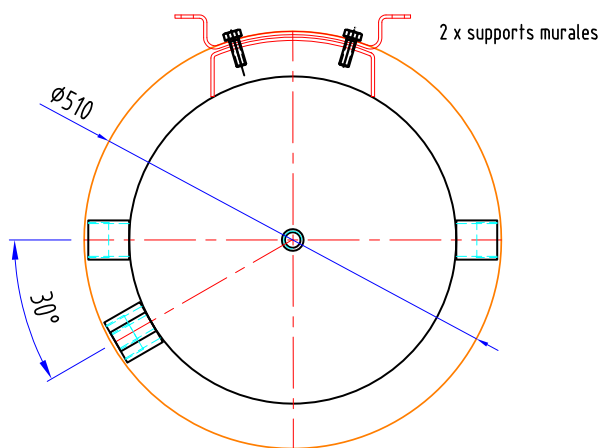
STA PUFFER 100 L sol/mural 8 piquages
