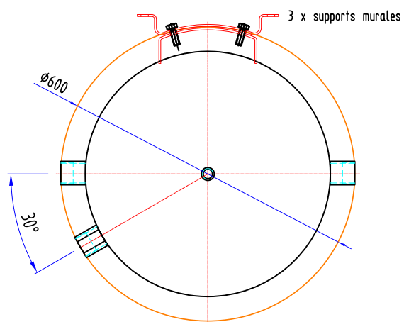
STA PUFFER 200 L sol/mural 8 piquages
