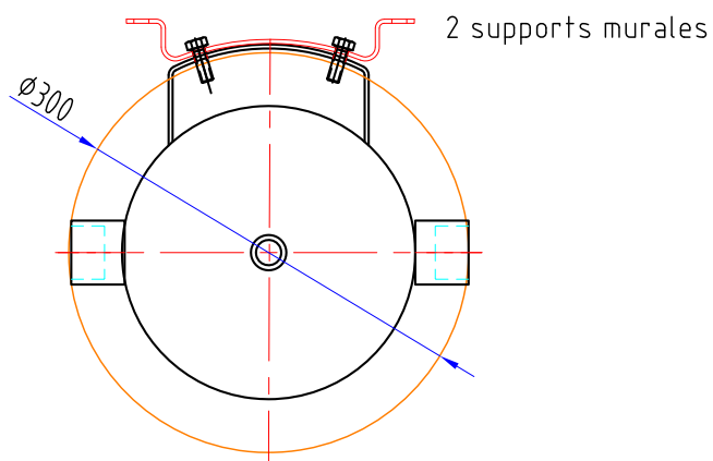
STA PUFFER 15 L mural 4 piquages
